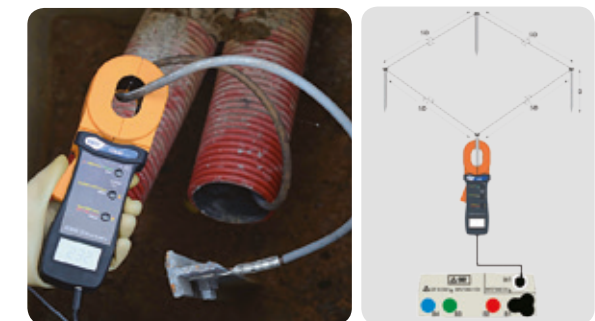
Measurement with clamp T2100
